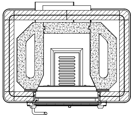
SECTION C-C SCALE 1 : 12
