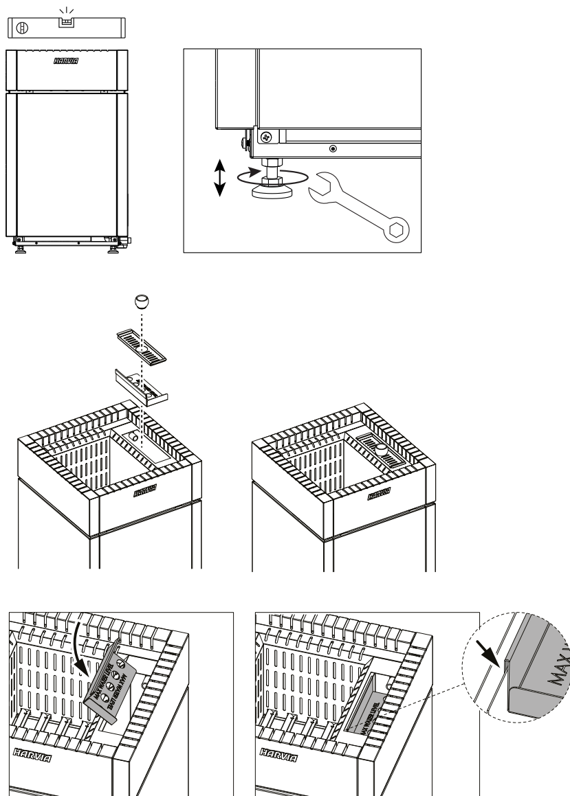
Figure 2. Sauna heater installation
