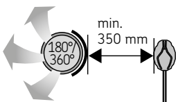
Figure 9. Minimum distance from the supply air vent to the temperature sensor
